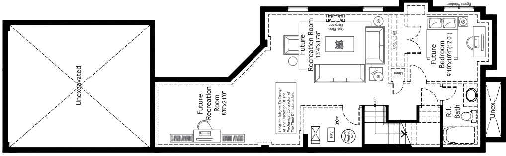
Basement Plan
